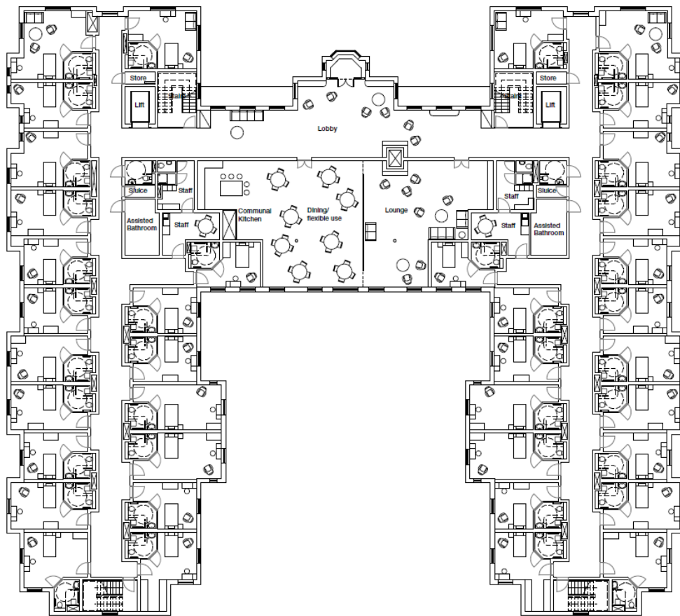
Approved First Floor Plan
